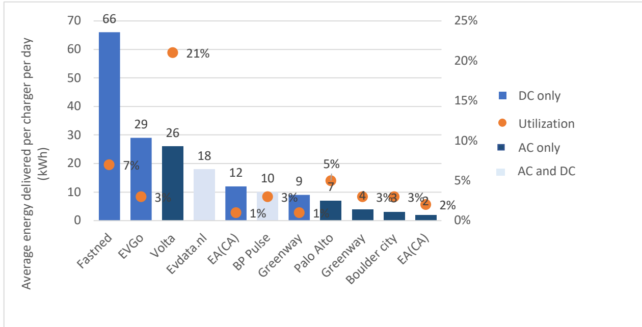
Figure 11.25: Average energy delivered per day per charger by different charge point operators in USA and Europe along with their utilization (based on Bloomberg’s data).
