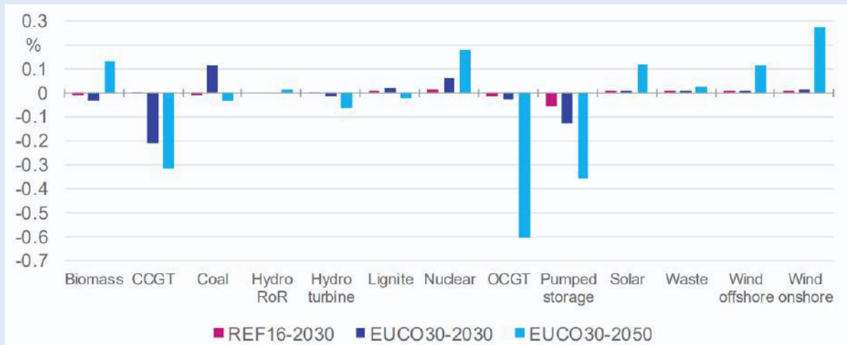
Figure 5.13: Difference in generation between RTP- and base scenario for EU countries (Klettke and Mose 2018)
