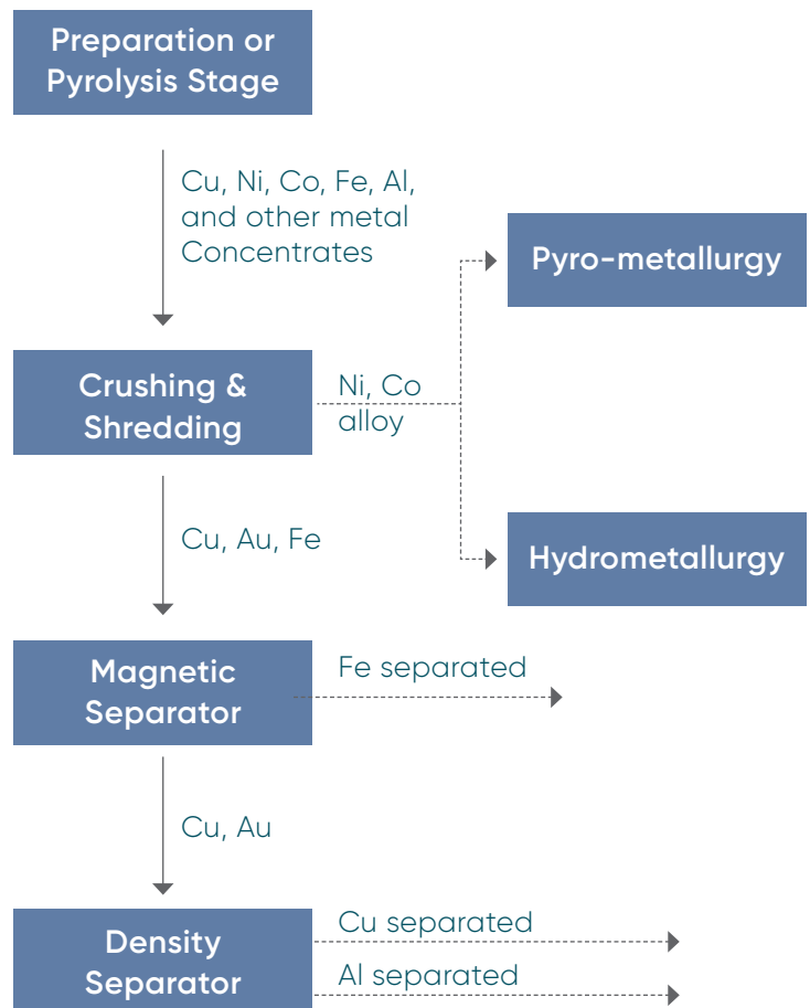
Figure 2: Mechanical recycling process
