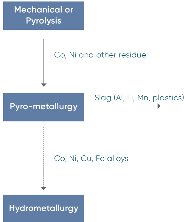
Figure 3: The pyro-metallurgy recycling process
